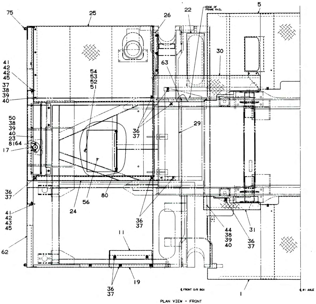
PLAN VIEW - FRONT
